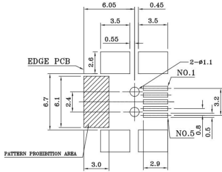
RECOMMENDED PCB PATTERN LAYOUT
