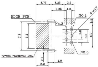
RECOMMENDED PCB PATTERN LAYOUT
