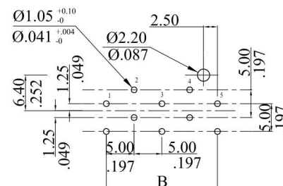
PCB special layout for 5011P**VV(W)**
