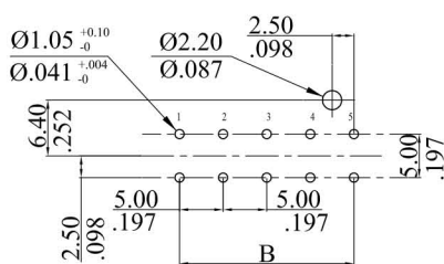
PCB layout for 5011P**VT(S)**
