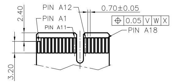
ADD-IN CARD EDGE-FINGER DIMENSIONS DEFAULT TOLERANCE ±0.05
