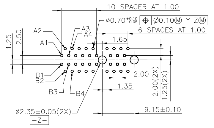
RECOMMENDED FOOTPRINT(TOP VIEW) DEFAULT TOLERANCE ±0.05
