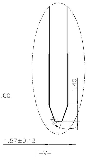
DETAIL "A" SCALE 4/1
