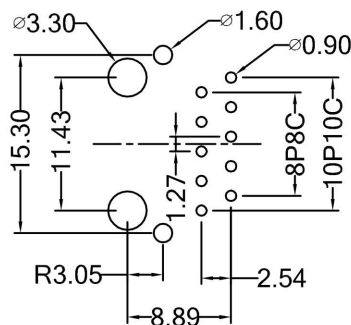
R3.05 PCB LAYOUT / TOP VIEW
