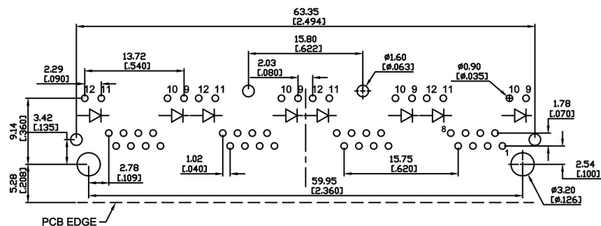
SUGGESTED PCB LAYOUT TOP VIEW
