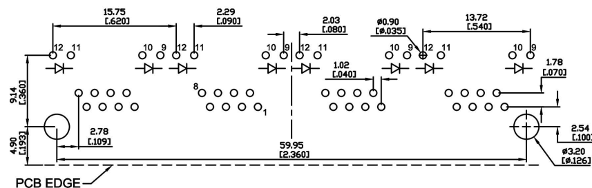
SUGGESTED PCB LAYOUT TOP VIEW
