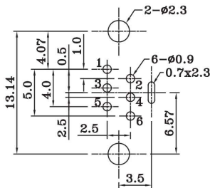
COMPONENT SIDE (PCB LAYOUT)
