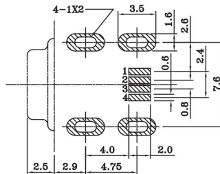
COMPONENT SIDE PCB LAYOUT
