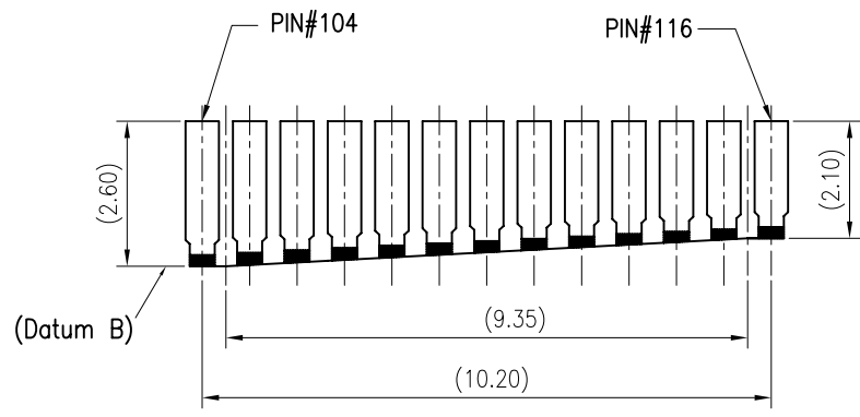
Figure 7 Step and ramp dimensions
