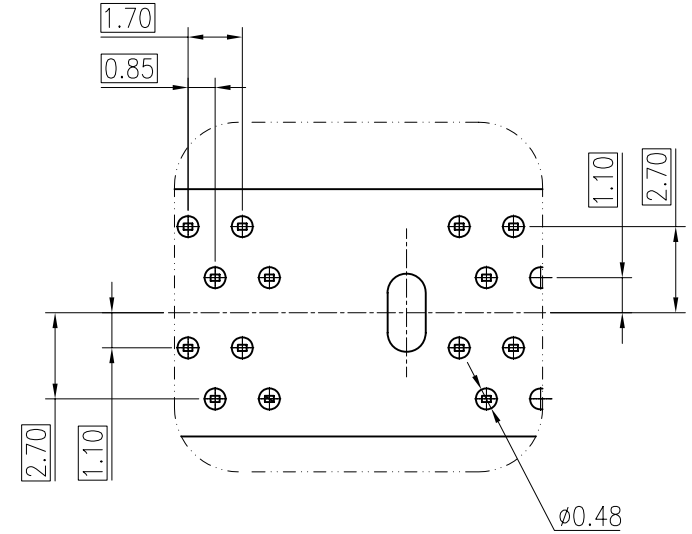
OUTER LOCUS OF CONNECTOR SOLDER PIN TAILS SCALE 5:1
