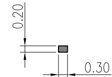
SOLDER TAIL SECTION SECTION B-B(10:1)
