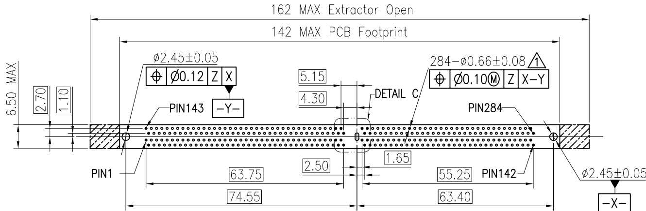
RECOMMENDED PCB LAYOUT(CONNECTOR SIDE) (TOL.:±0.05)
