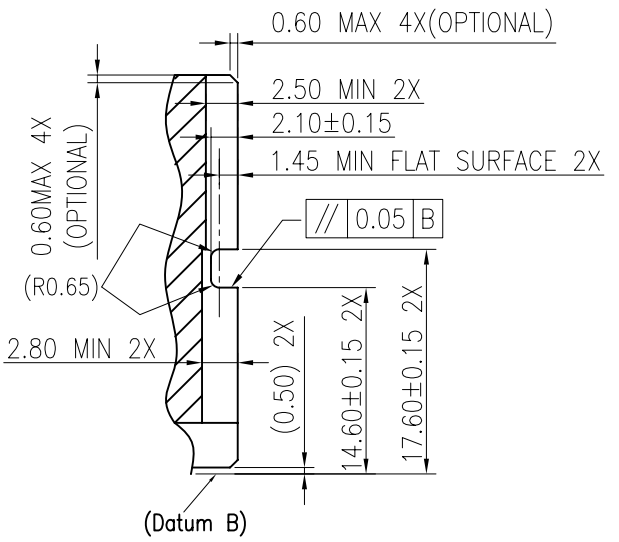
DETAIL G Figure 6 Module outline
